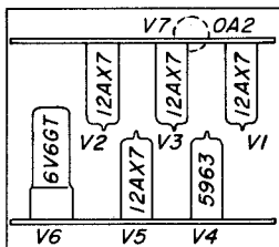
Figure 7. Tube Location Chart (rear view of the instrument) for Type 1263-B Amplitude-Regulating Power Supply.
