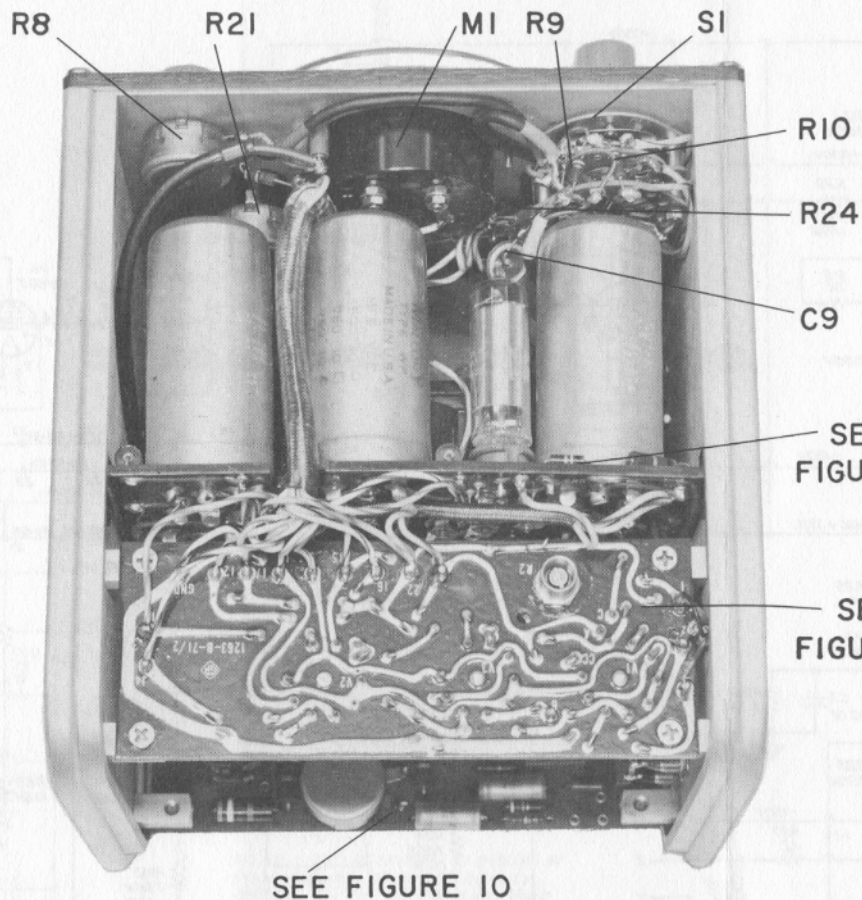
Figure 9. Top Interior View of the Type 1263-B Amplitude-Regulating Power Supply.
